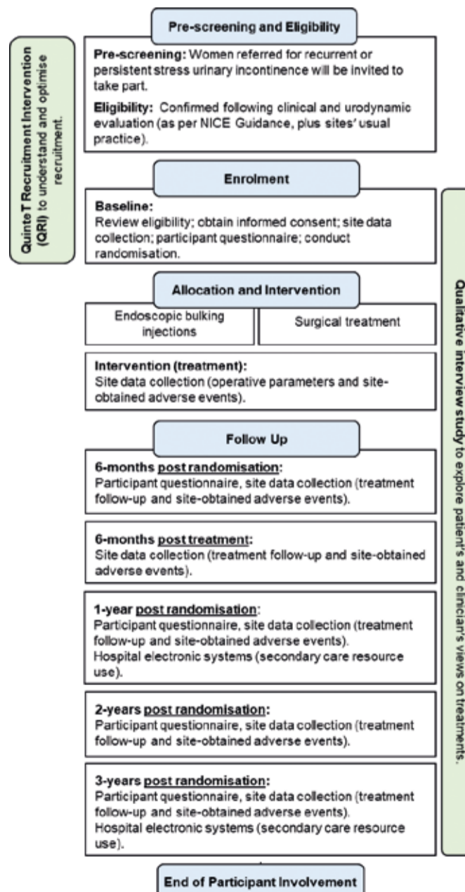
Figure 1: Trial flowchart
